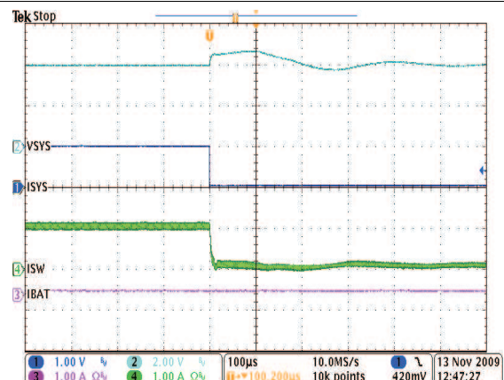
0-A - 1-A Transient on V sys V BUS = 5.5 V No Battery V OREG = 4 V I CHARGE = 950 mA I IN_limit = 975 mA
