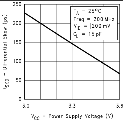
Figure 9. Differential Skew vs Power Supply Voltage
