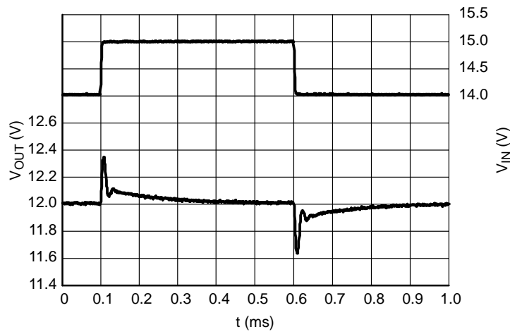
Figure 33. Line Transients, 12.0 V Version, t_R = t_F = 5 \mu\text{s} , I_{OUT} = 30 \text{ mA}
