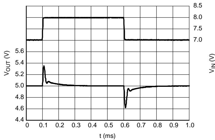
Figure 32. Line Transients, 5.0 V Version, t_R = t_F = 5 \mu\text{s} , I_{OUT} = 30 \text{ mA}
