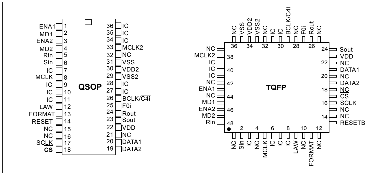
Figure 2 - Pin Connection
