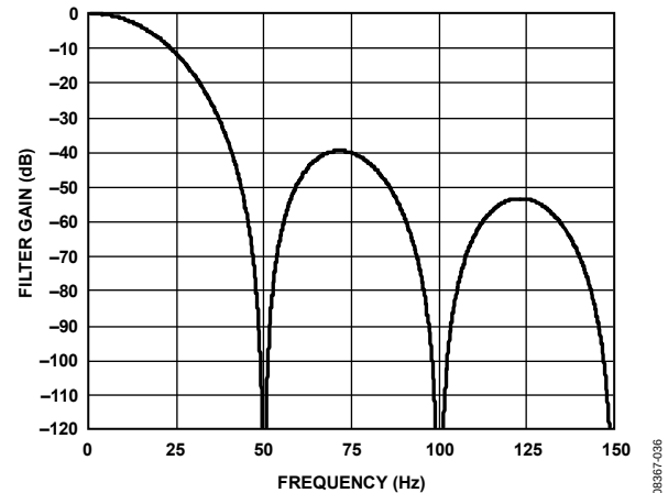
Figure 40. Sinc 3 Filter Response (FS[9:0] = 96)
