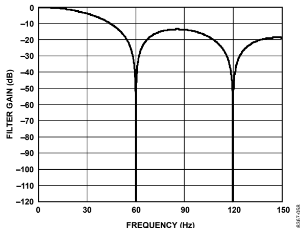
Figure 58. Filter Response for Average + Decimate Filter (Sinc 4 Filter, FS[9:0] = 5, Average by 16)
