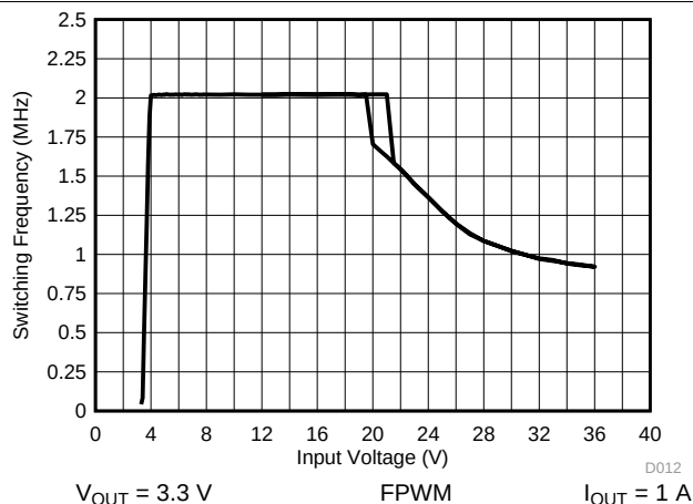
Figure 48. Switching Frequency vs Input Voltage
