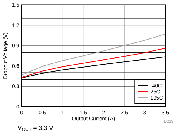
Figure 46. Dropout for \geq 1.85 \text{ MHz}
