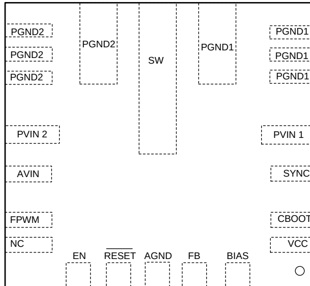
RNL Package 22-Pin VQFN Top View
