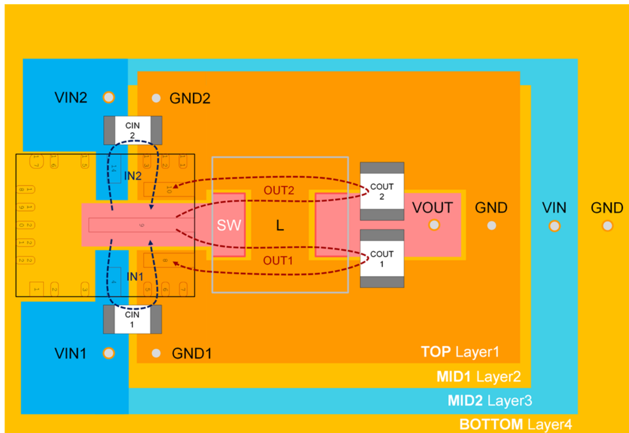
Figure 59. Layout of the Power Components and Current Flow
