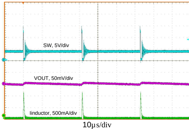
Figure 16. Typical PFM Switching Waveforms
