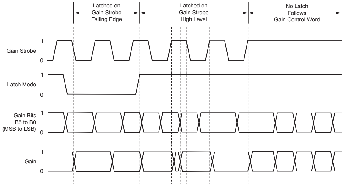
Figure 43. Gain Mode Timing
