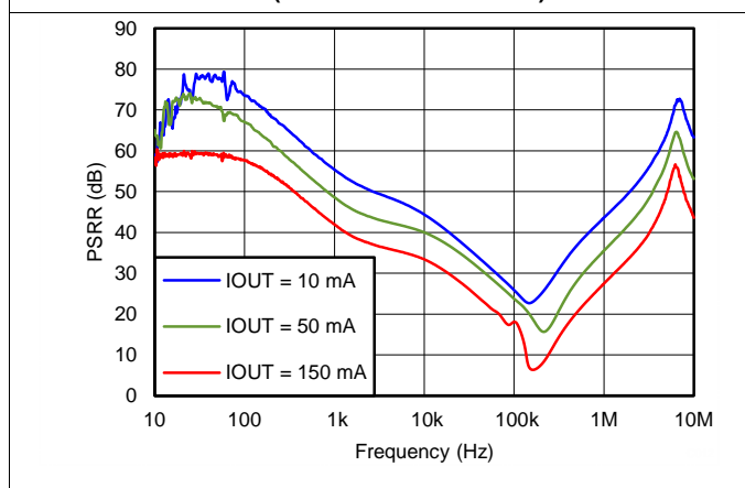
Figure 11. Power-Supply Rejection Ratio vs Frequency ( V_{OUT} = 3.3\text{ V} )
