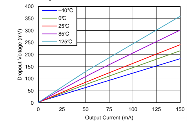
Figure 8. Dropout Voltage vs I_{OUT} ( V_{OUT} = 3.3\text{ V} )
