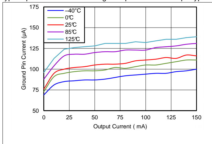
Figure 7. Ground Pin Current vs I_{OUT}
