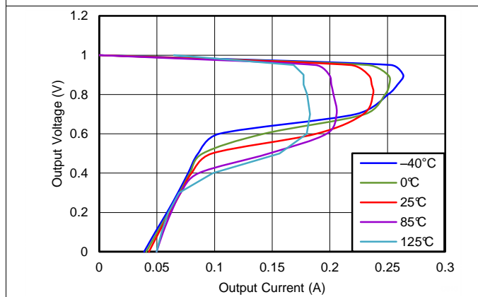
Figure 9. Output Voltage vs Output Current ( V_{OUT} = 1\text{ V} ) (Foldback Current Limit)
