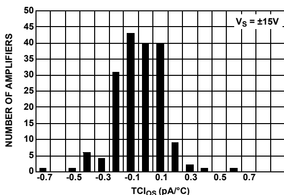
FIGURE 19. TC_{IOS-} vs NUMBER OF AMPLIFIERS, V_S = \pm 15V
