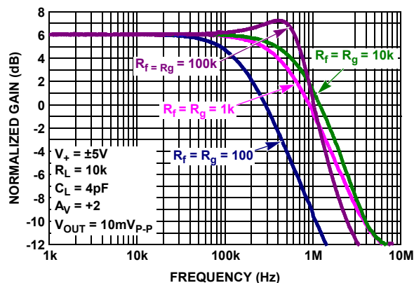
FIGURE 42. FREQUENCY RESPONSE vs FEEDBACK RESISTANCE R_f/R_g
