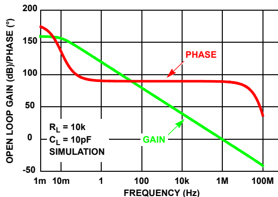
FIGURE 67. SIMULATED OPEN-LOOP GAIN, PHASE vs FREQUENCY
