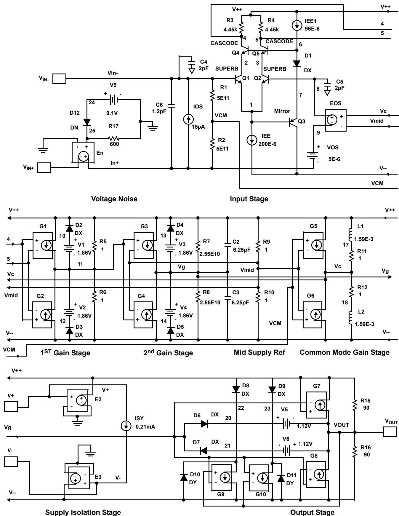
FIGURE 56. SPICE SCHEMATIC
