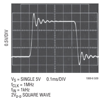
Transient Response
