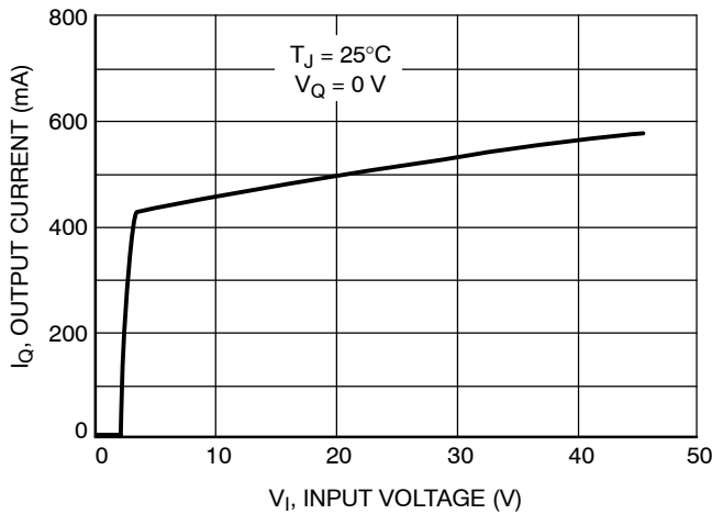
Figure 39. Maximum Output Current vs. Input Voltage
