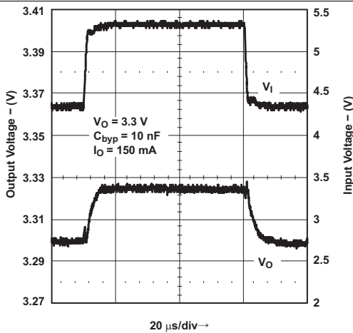
Figure 25. Line Transient Response
