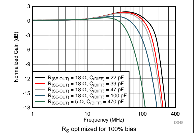
Figure 48. Frequency Response Across Capacitive Load
