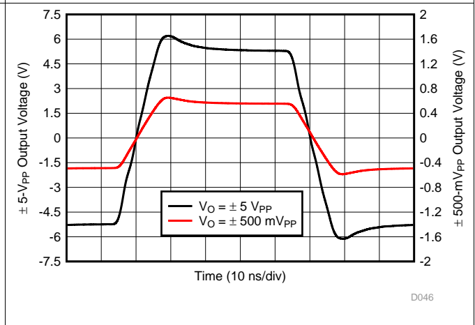
Figure 46. Pulse Response
