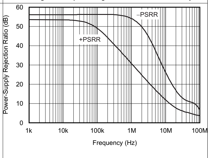
Figure 16. PSRR vs Frequency
