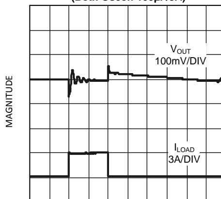
Load Transient Response (Both Oscon 100 \mu\text{F}/3\text{A} )
