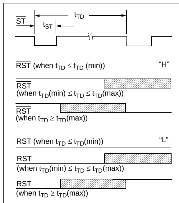
FIGURE 4-8: Strobe Input.
