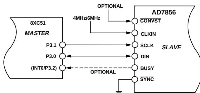
Figure 37. 8XC51/PIC16C42 Interface
