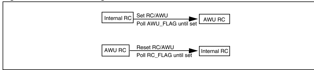
Figure 9. Clock switching
