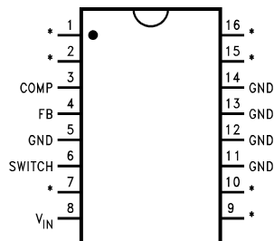
Figure 3. Top View Order Number LM2577N-12, LM2577N-15, or LM2577N-ADJ See NS Package Number N16A
