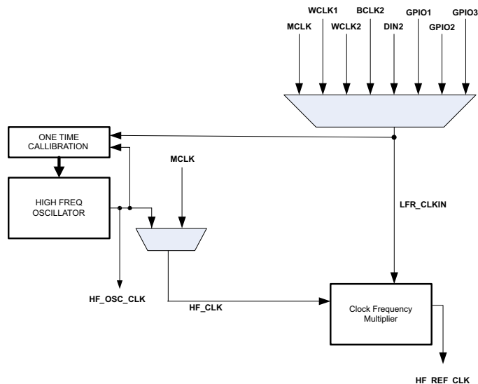
Figure 63. Low-Frequency Clocking
