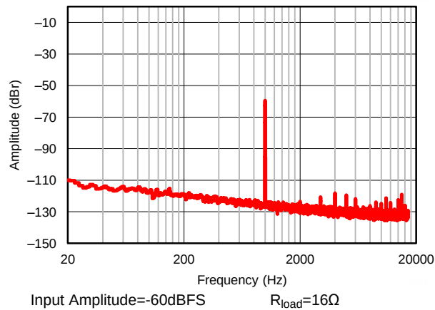
Figure 25. DAC Playback on Headphone Amplifier, Output Amplitude versus Frequency
