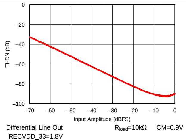
Figure 20. DAC Playback on Line Out Amplifier, Total Harmonic Distortion + Noise versus Input Amplitude
