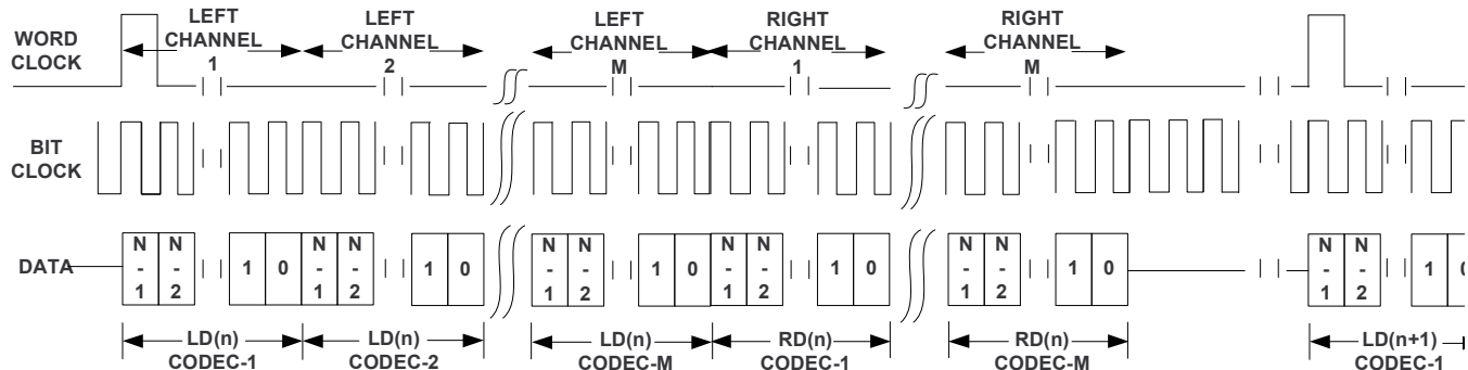
Figure 101. DSP Timing for Multiple Devices Interfaced Together, Grouped Left Channels and Right Channels
