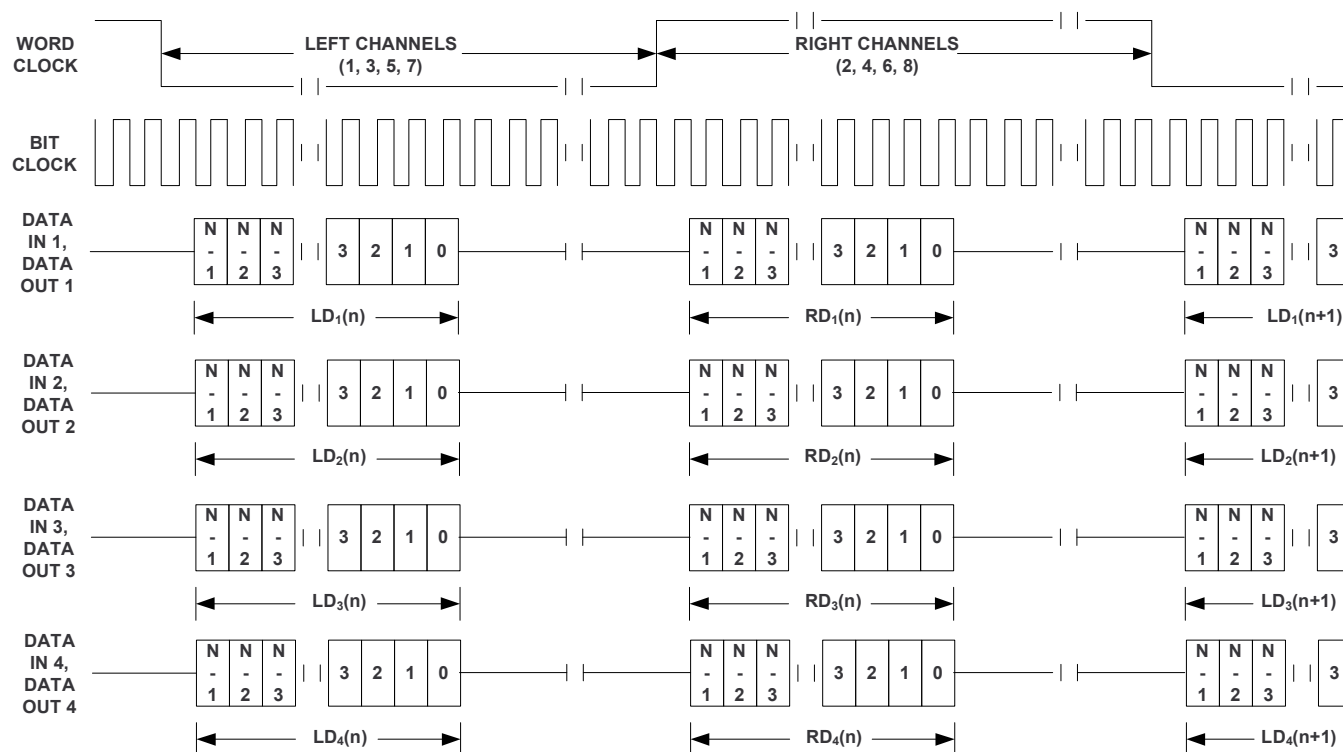
Figure 106. I²S Timing for Multi-channel Mode, Four Data Lines
