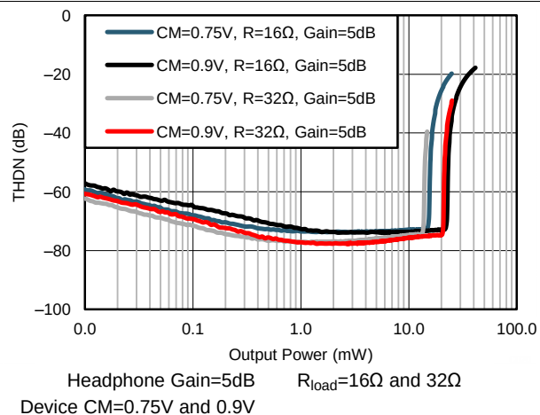
Figure 27. DAC Playback on Headphone Amplifier, Total Harmonic Distortion + Noise versus Output Power
