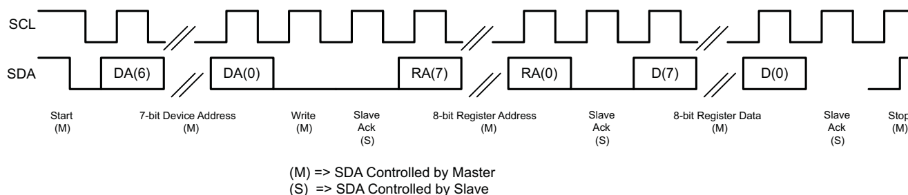
Figure 78. I 2 C Write
