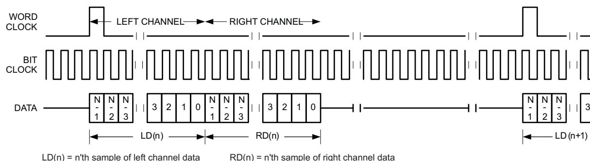
Figure 93. Timing Diagram for DSP Mode
