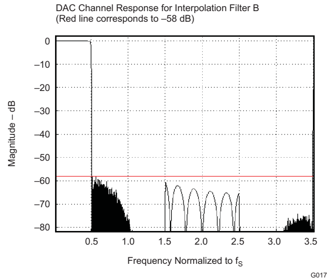
Figure 56. Channel Interpolation Filter B, Frequency Response
