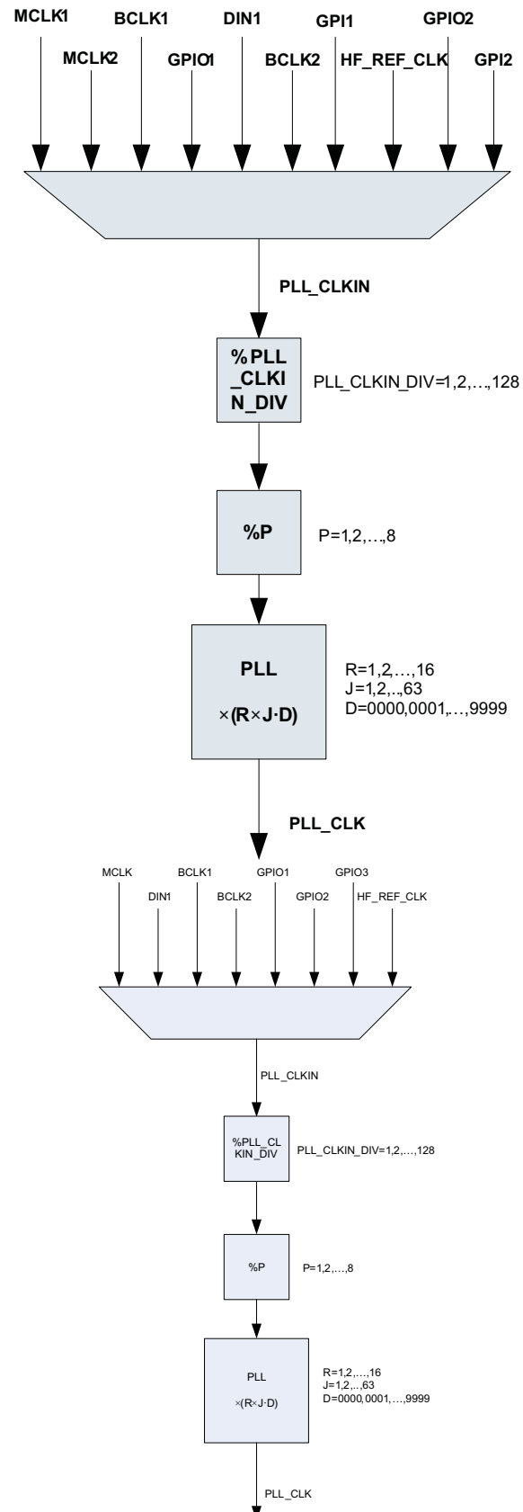
Figure 62. PLL Clocking and Mux
