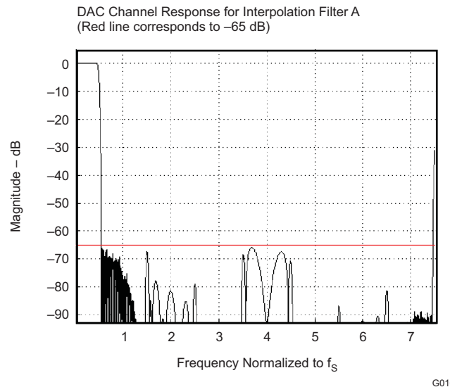
Figure 55. DAC Interpolation Filter A, Frequency Response
