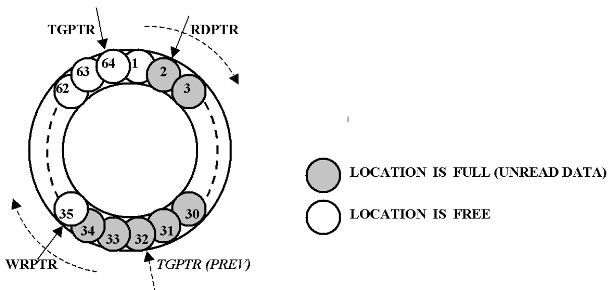
Figure 71. Circular Buffer
