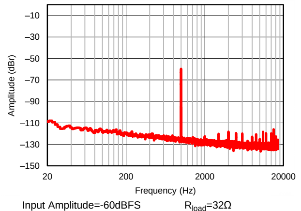
Figure 26. DAC Playback on Headphone Amplifier, Output Amplitude versus Frequency
