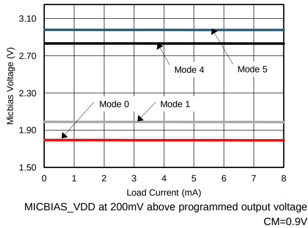
Figure 18. Micbias, Output Voltage versus Load Current
