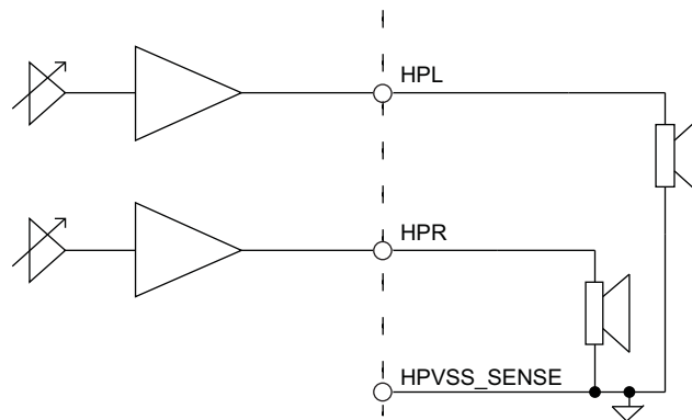
Figure 38. TLV320AIC3268 Ground-Centered Headphone Output
