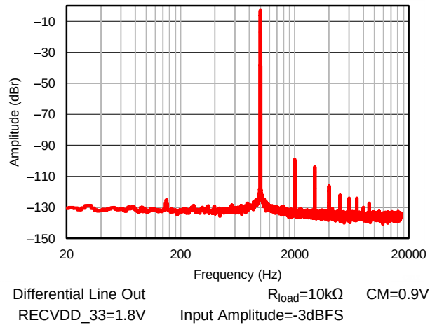
Figure 19. DAC Playback on Line Out Amplifier, Output Amplitude versus Frequency
