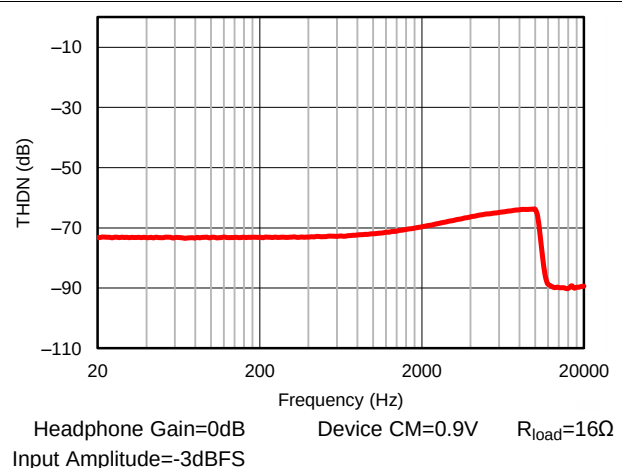
Figure 28. DAC Playback on Headphone Amplifier, Total Harmonic Distortion + Noise versus Input Frequency
