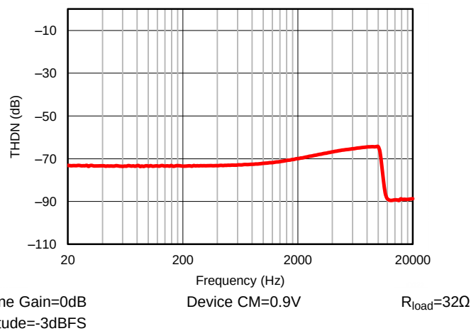
Figure 29. DAC Playback on Headphone Amplifier, Total Harmonic Distortion + Noise versus Input Frequency
