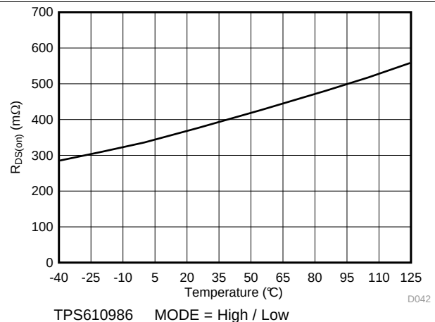
Figure 16. Low Side Switch on Resistance vs Temperature
