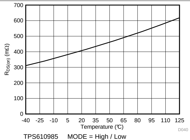
Figure 14. Low Side Switch On Resistance vs Temperature
