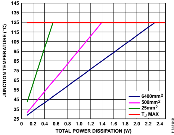
Figure 52. LFCSP, T A = 25°C
