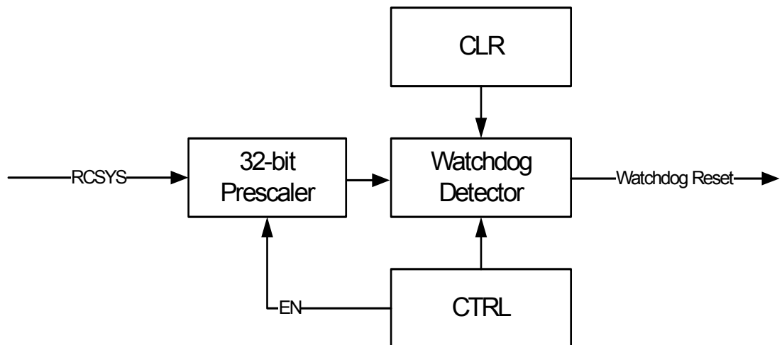
Figure 11-1. WDT Block Diagram
