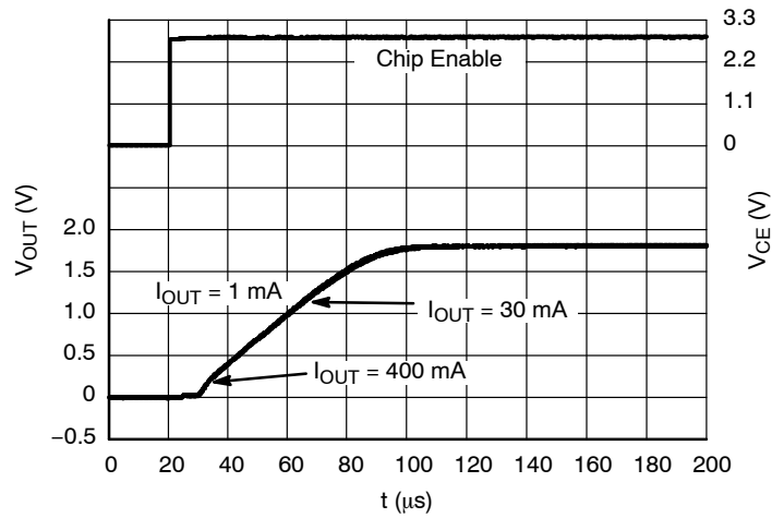
Figure 41. Start-up, 1.8 V Version, V_{IN} = 2.8 V
