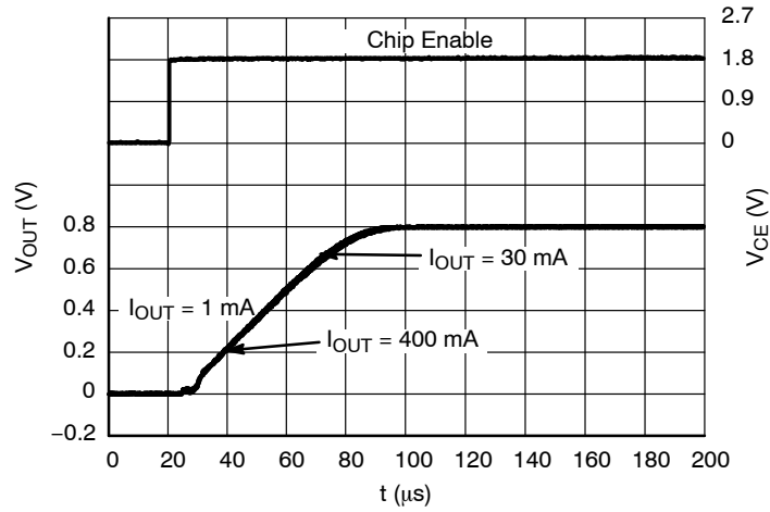
Figure 39. Start-Up, 0.8 V Version, V_{IN} = 1.8 V
