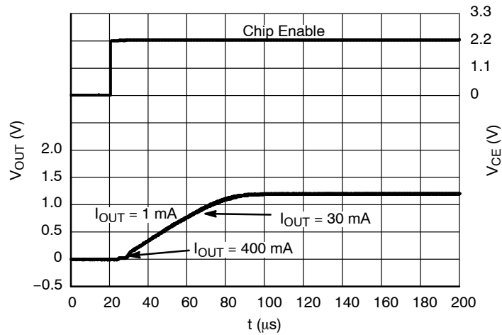
Figure 40. Start-Up, 1.2 V Version, V_{IN} = 2.2 V
