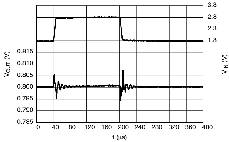
Figure 27. Line Transients, 0.8 V Version, t_R = t_F = 5 \mu s , I_{OUT} = 30 \text{ mA}
