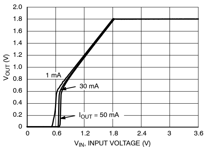
Figure 20. Output Voltage vs. Input Voltage, 1.8 V Version
