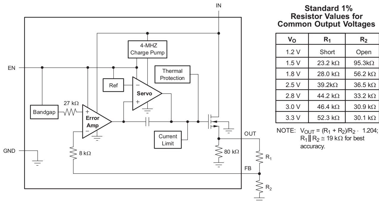
Figure 30. Adjustable-Voltage Version
