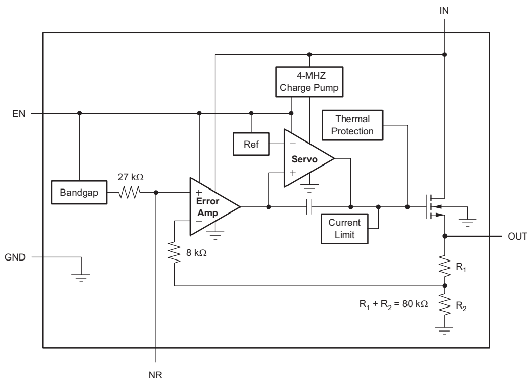
Figure 29. Fixed-Voltage Version
