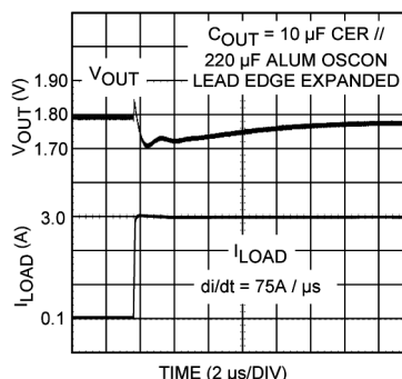
Figure 22. 10-μF Ceramic Paralleled by 220-μF OSCON
