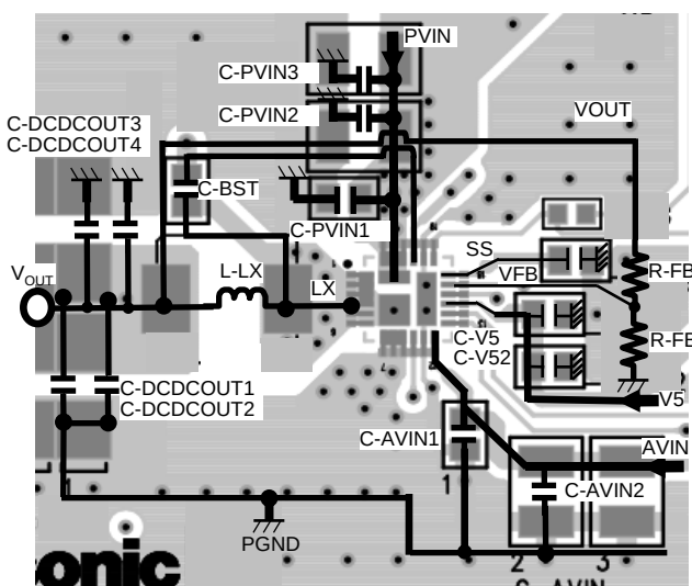
Figure : layout
