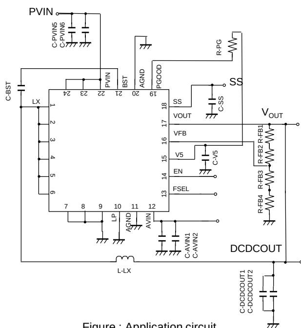
Figure : Application circuit
