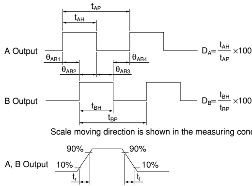
Fig.1 Output Waveforms
