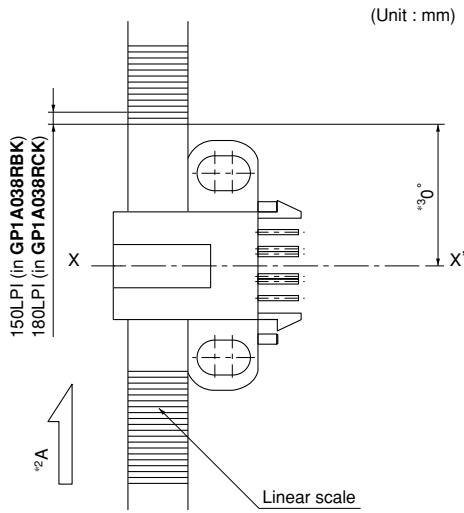
Fig.4 Measuring Condition
