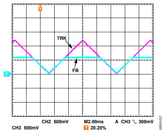
Figure 26. Tracing Function
