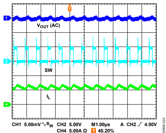
Figure 23. Steady Waveform
