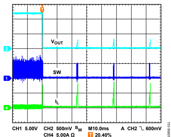
Figure 24. Output Short
