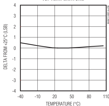
CHANGE IN ADC OFFSET vs. TEMPERATURE
