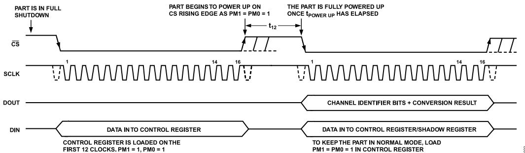
Figure 22. Full Shutdown Mode Operation
