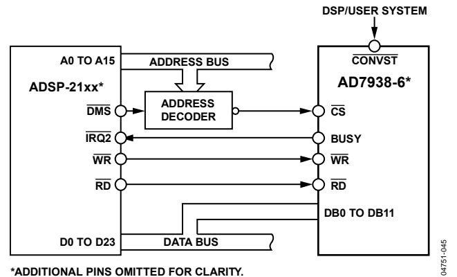
Figure 43. Interfacing to the ADSP-21xx
