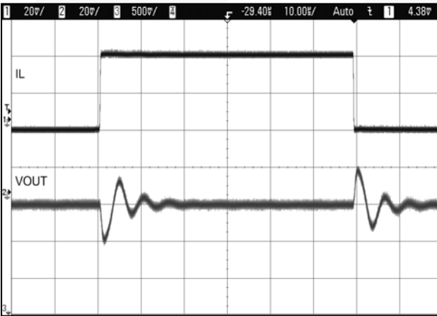
Figure 24. Load Transient, 0 mA to 400 mA, V_{OUT} = 2.5\text{ V} in High-Power Mode
