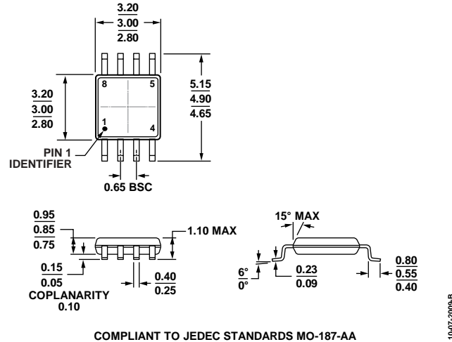
COMPLIANT TO JEDEC STANDARDS MO-187-AA Figure 75. 8-Lead Mini Small Outline Package [MSOP] (RM-8) Dimensions shown in millimeters
