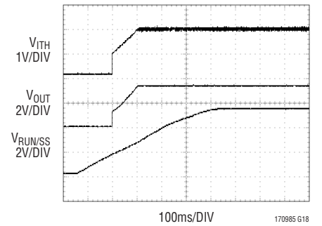
Soft-Start Up
