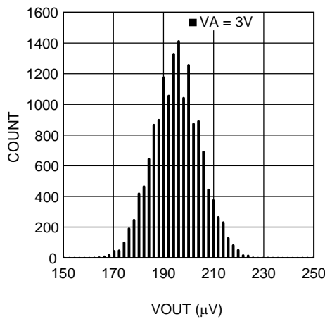
Figure 14. Histogram Without Calibration at Gain = 1
