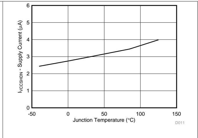
Figure 11. VIN Shutdown Current vs Junction Temperature
