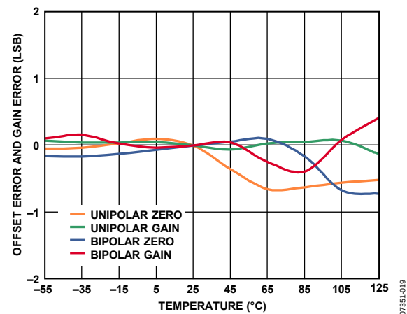
Figure 19. Offset and Gain Errors vs. Temperature
