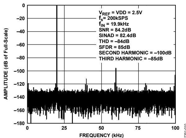
Figure 10. 20 kHz FFT, V_{REF} = V_{DD} = 2.5\text{ V}
