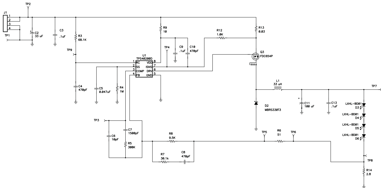
Figure 47. Wide Input Voltage-Range LED Driver
