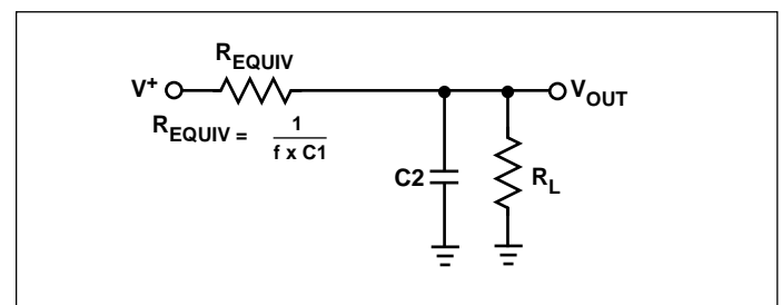
Figure 2b. Equivalent Output Resistance
