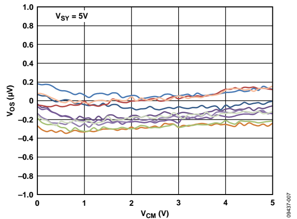
Figure 13. Input Offset Voltage vs. Common-Mode Voltage
