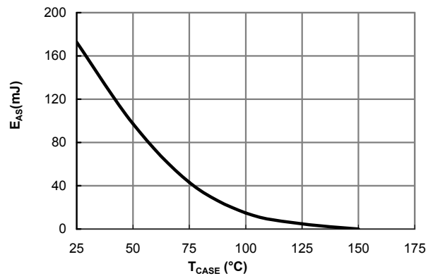
Figure 12: Avalanche energy
