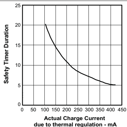
Figure 2. DTC Operation
