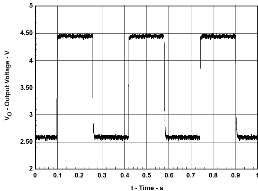
Figure 15. Battery-Absent Detection Waveforms
