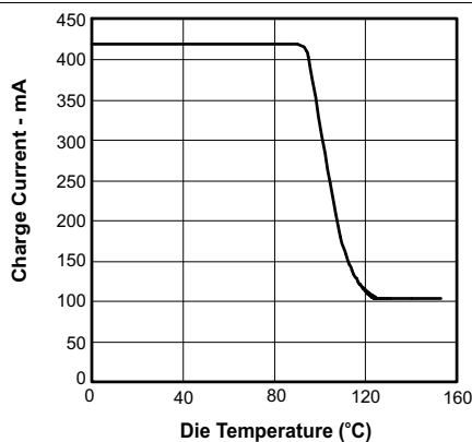
Figure 1. Thermal Regulation
