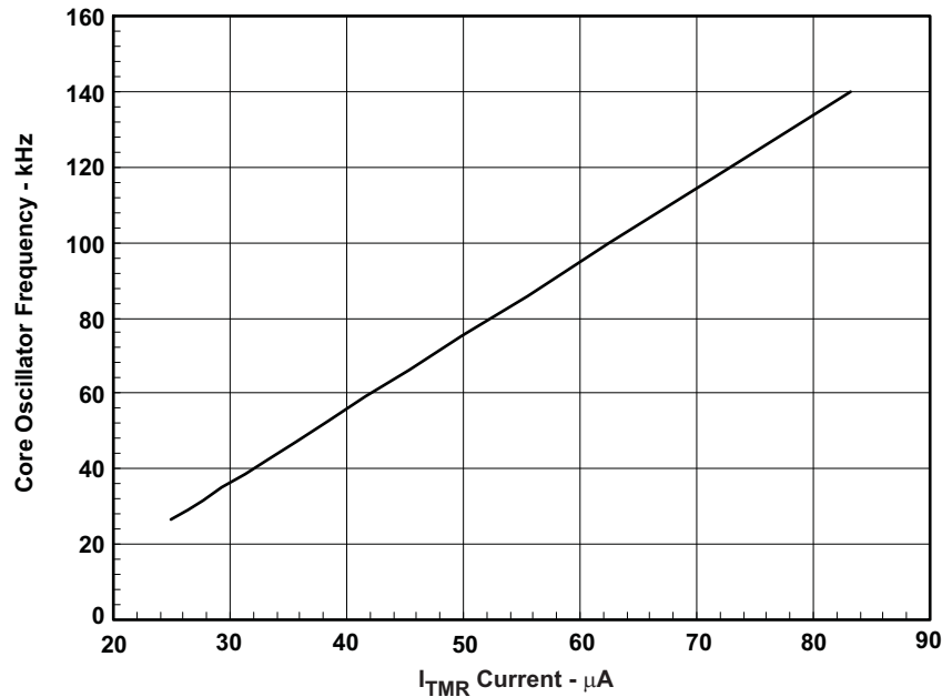
Figure 14. bq24085/6/7/8 Oscillator Linearity vs I_{TMR} R_{TMR} 30 K \Omega – 100 K \Omega
