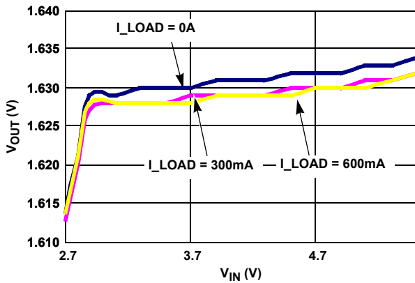
FIGURE 3. LINE REGULATION
