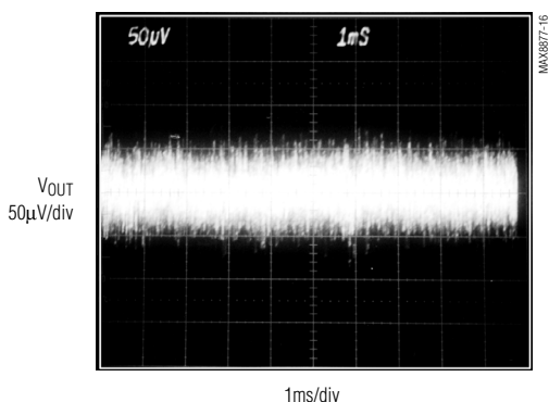
MAX8877_EUK25, C_{OUT} = 10\mu F , I_{LOAD} = 10mA , C_{BP} = 0.1\mu F
