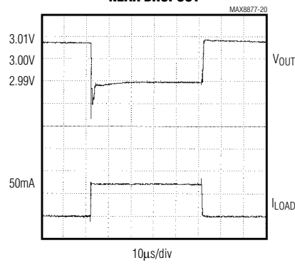
MAX8877_EUK30, V_{IN} = V_{OUT} + 0.1V , C_{IN} = 10\mu F , I_{LOAD} = 0mA TO 50mA
