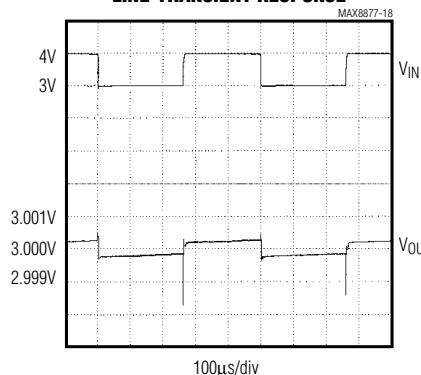
MAX8877_EUK30, I_{LOAD} = 50mA
