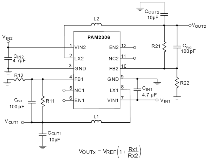
Figure 1. Adjustable Voltage Regulator
