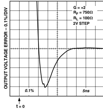
TPC 28. Settling Time, V_S = \pm 5 V
