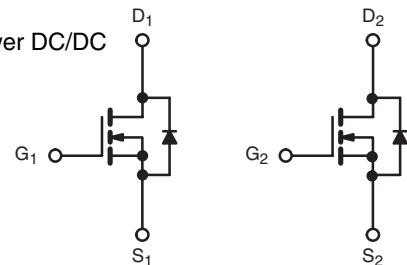
N-Channel MOSFET
