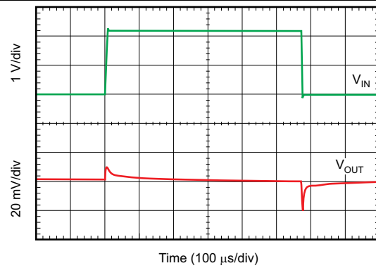
Figure 50. Line Transient Response
