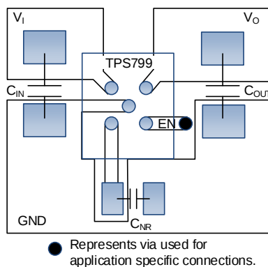
Figure 31. Layout Example
