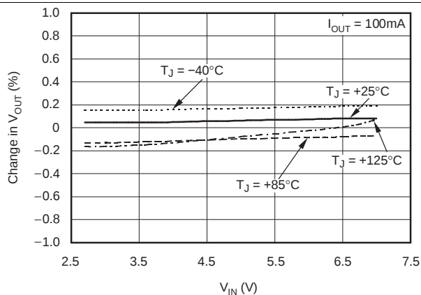
Figure 2. Line Regulation
